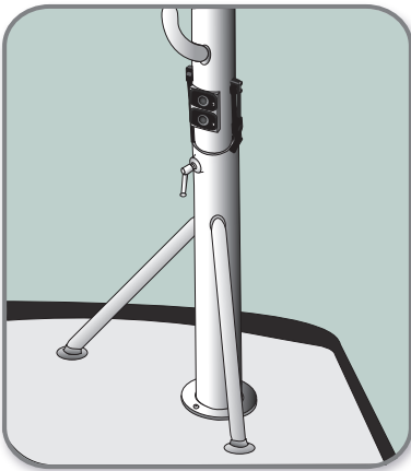
"DECK-STEPPED MOUNTING"
