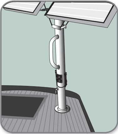
"THROUGH-THE-DECK MOUNTING"
