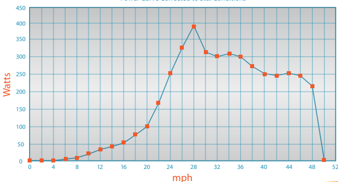
Air-X Power Curve
