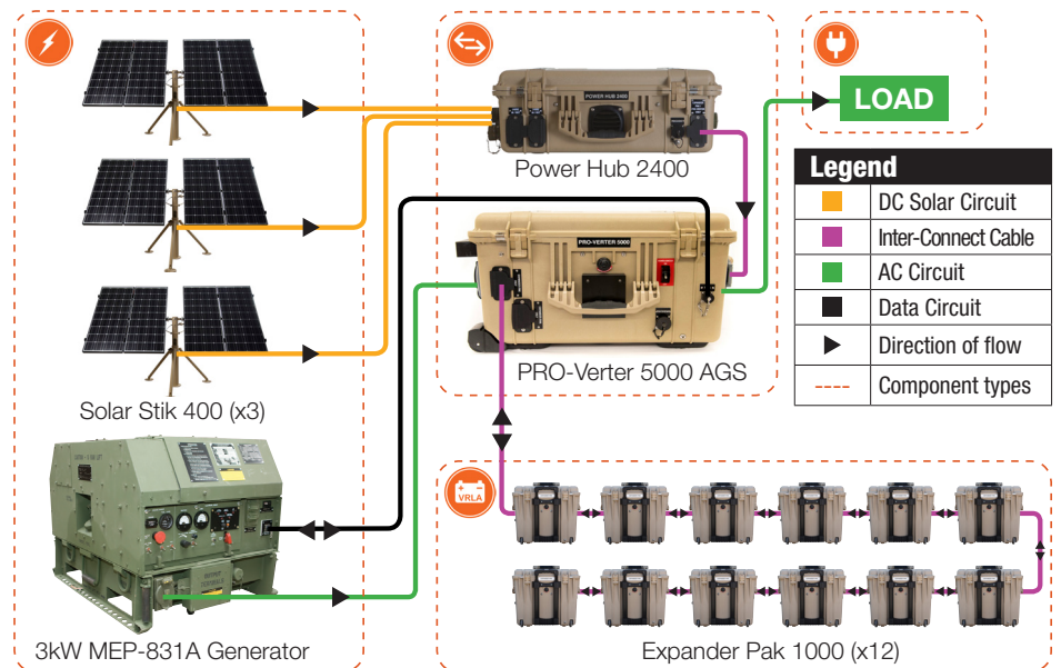
Figure 4 - The Solar Stik 3.0 kW TQG Hybrid Power System
